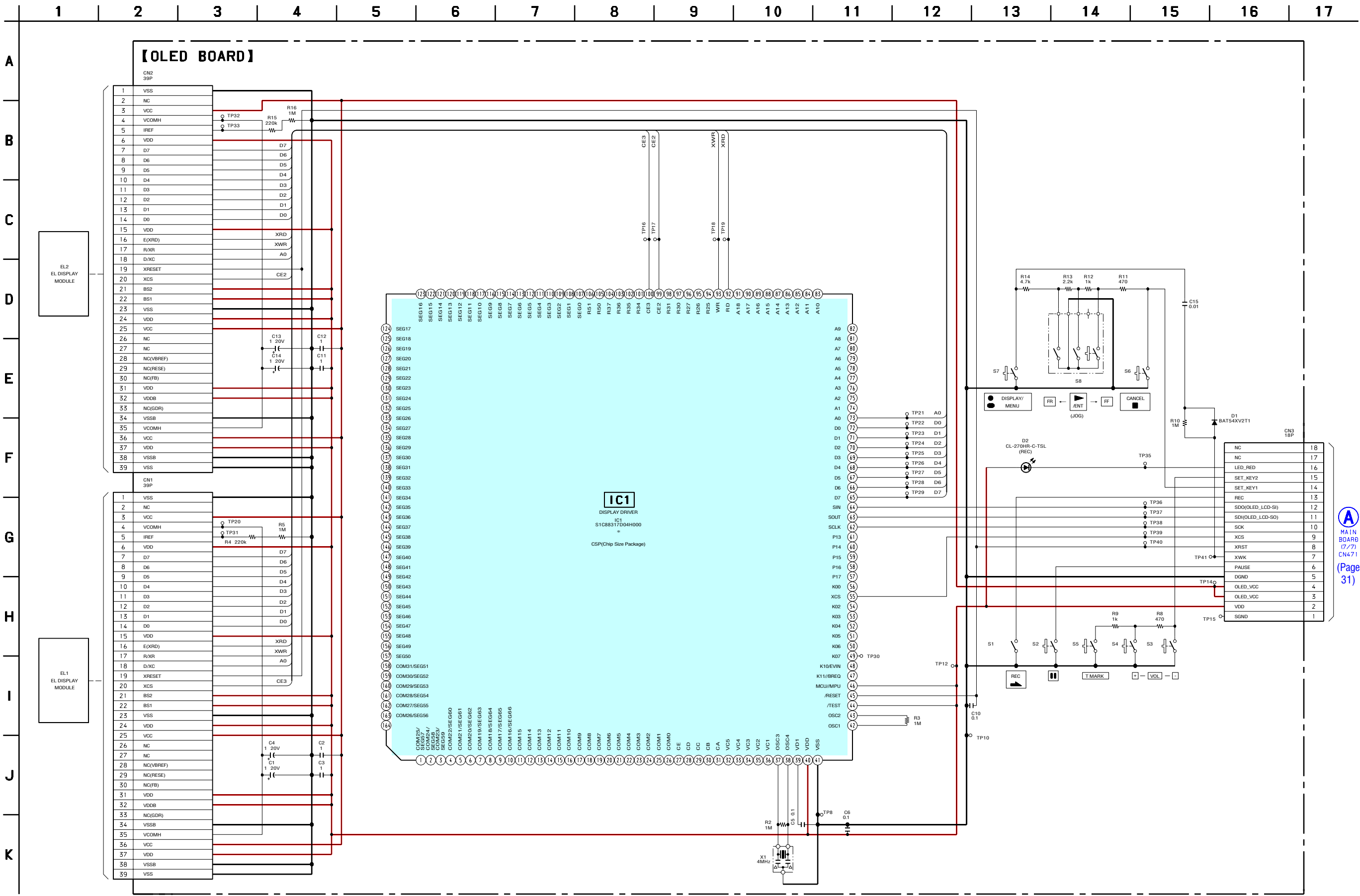
6-14. SCHEMATIC DIAGRAM – OLED Board – • See page 42 for IC Pin Function Description.
